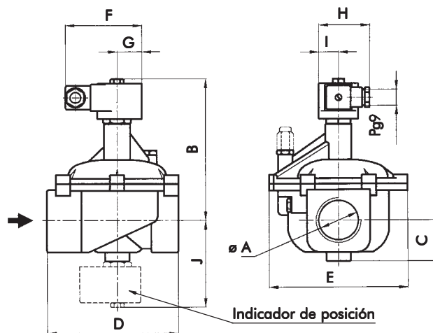
SERVODIAPHRAGMA
